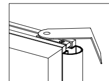
YHC 7 HEADER HOOK To be used with 11 13/16" flush mount headers
